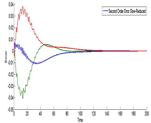
Figure 5.6: Error between the slow motions of the system in the singular perturbation form and of the aggregate model
