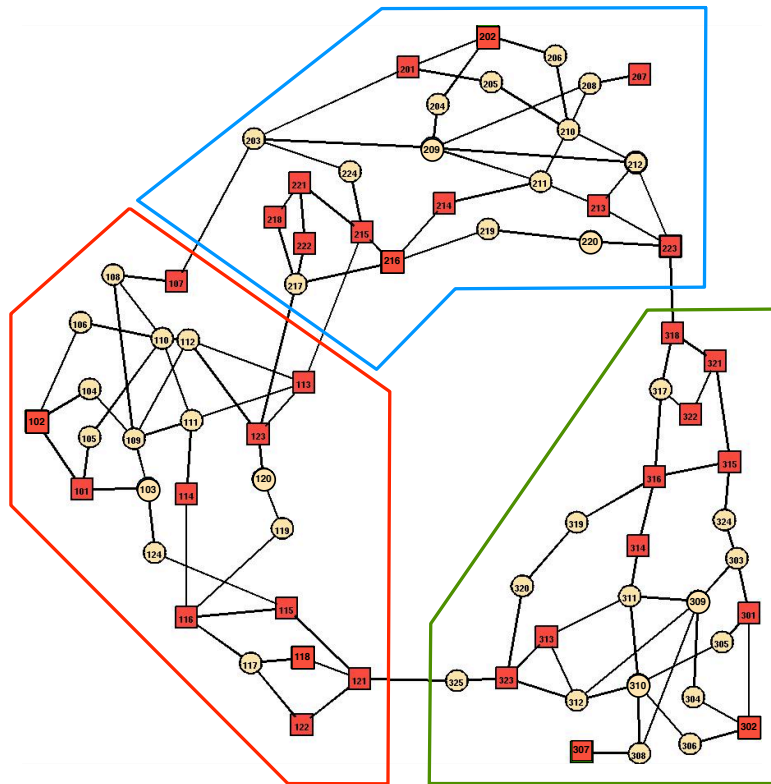
Figure 5.1: Illustration of RTS 96 power network with three areas. Here the square nodes are the generators and the circles the load buses of the network.
