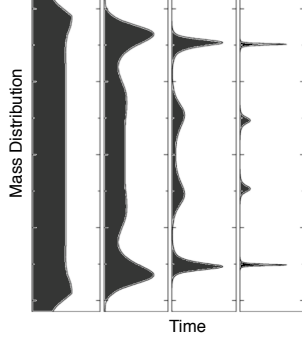
FIG. 4.1. A schematic illustration of convergence of an Eulerian HK system with no input in the weak-star topology to an atomic measure, whose atoms are separated by a distance greater than r .
