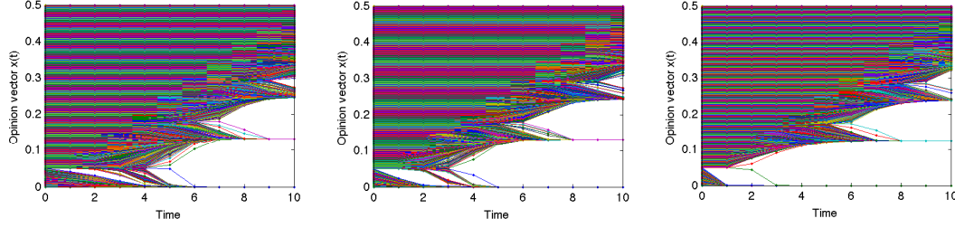
FIG. 5.1. Evolutions of Eulerian HK systems with uniform initial distribution \mu_0 \sim \mathcal{U}(-L, L) and input u = w\delta_0 are illustrated. We consider \rho_0 = 1 , L \in \mathbb{R}_{>0} and sufficiently larger than r = 0.05 , and three values of \frac{r}{r+w} = 0.7, 0.3, 0.01 (from left to right). To assure lucidity of results, the agent based behavior of descrittized Eulerian HK systems is represented. Simulating this system for various values of \frac{r}{r+w} , we conjecture that Assumption 5.1 holds for all t \geq 5 and Assumption 5.2 is always satisfied. Moreover, it can be observed that for a larger w (i.e., a more strict report of the message) a smaller population will be attracted to the input's center and the rest will cluster away from the input.
