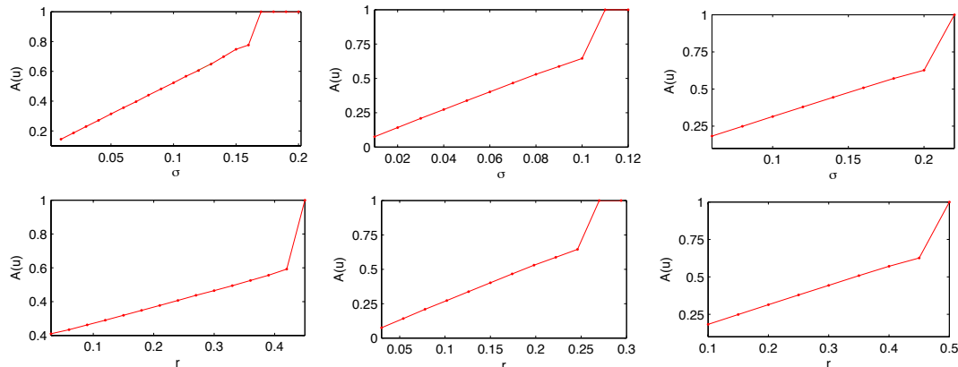
FIG. 5.2. In evolutions of Eulerian HK systems with uniform initial distribution \mu_0 \sim \mathcal{U}(-x_0, x_0) and input u \sim \mathcal{N}(0, \sigma^2) , the attracted population \mathcal{A}(r, u, \mu_0) is found for different values of the following parameters: \sigma , x_0 , and r . In conclusion, for \sigma \leq 0.05|\text{supp } \mu_0| and r \leq 0.125|\text{supp } \mu_0| , the simulations reveal the following linear relation: \mathcal{A}(r, u, \mu_0) \simeq (8\sigma + 2r)/|\text{supp } \mu_0| . In the top left plot, x_0 = 1 , r = 0.1 , and \sigma \in \{0.01, 0.02, \dots, 0.17\} ; in the bottom left, x_0 = 1 , \sigma = 0.04 , and r \in \{0.03, 0.06, \dots, 0.45\} ; in the middle, x_0 = 1 and (\sigma, r) \in \{(0.01, 0.03), \dots, (0.12, 0.3)\} ; and in the right, x_0 = 2 and (\sigma, r) \in \{(0.06, 0.1), \dots, (0.22, 0.5)\} .
