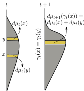
FIG. 2.1. A schematic illustration of push forward of a measure \mu_t via the flow map \gamma_t .
