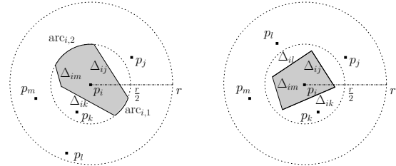
Fig. 2. The shaded regions are examples of sets V_i(\mathcal{P}) \cap B_{\frac{r}{2}}(p_i) .
