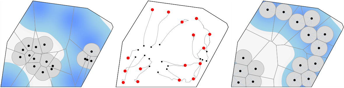
FIGURE 5. Area problem (with agent performance f(x) = 1_{[0, \frac{r}{2}]}(x) ): discrete-time algorithm T_{\text{is}} for 16 agents on a convex polygonal environment. The left (respectively, right) figure illustrates the initial (respectively, final) locations and Voronoi partition. The central figure illustrates the gradient ascent flow. For each agent i , the intersection V_i \cap \bar{B}(p_i, \frac{r}{2}) is plotted in light gray. After 18 seconds, the value of the multi-center function is approximately 6.28977 .
