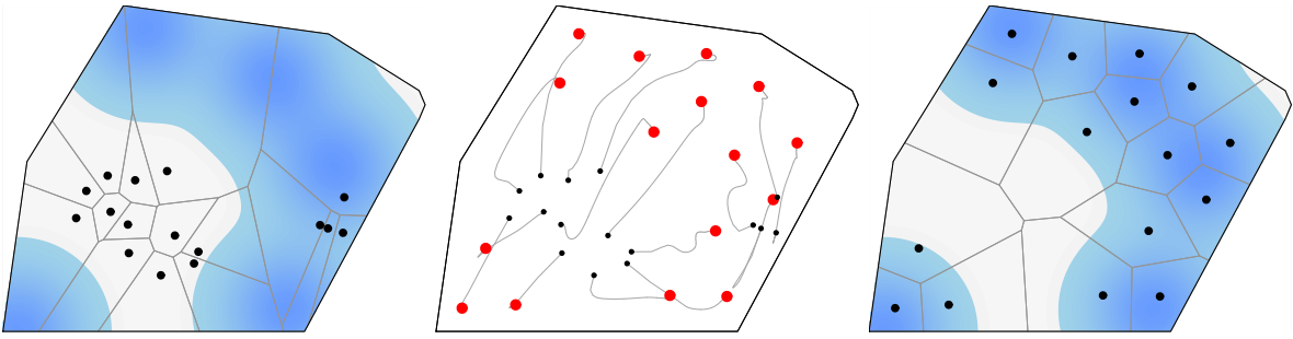
FIGURE 4. Centroid problem (with agent performance f(x) = -x^2 ): discrete-time algorithm T_{\text{is}} for 16 agents on a convex polygonal environment. The left (respectively, right) figure illustrates the initial (respectively, final) locations and Voronoi partition. The central figure illustrates the gradient ascent flow. After 90 seconds, the value of the multi-center function is approximately -.321531 .
