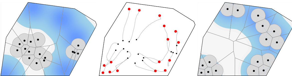
FIGURE 6. Mixed centroid-area problem (with continuous agent performance f(x) = -x^2 \mathbf{1}_{[0, \frac{r}{2}]}(x) - \frac{r^2}{4} \cdot \mathbf{1}_{[\frac{r}{2}, +\infty)}(x) ): discrete-time algorithm T_{\text{ls}} for 16 agents on a convex polygonal environment. The left (respectively, right) figure illustrates the initial (respectively, final) locations and Voronoi partition. The central figure illustrates the gradient ascent flow. For each agent i , the intersection V_i \cap \overline{B}(p_i, \frac{r}{2}) is plotted in light gray. After 90 seconds, the value of the multi-center function is approximately -0.252534 .
