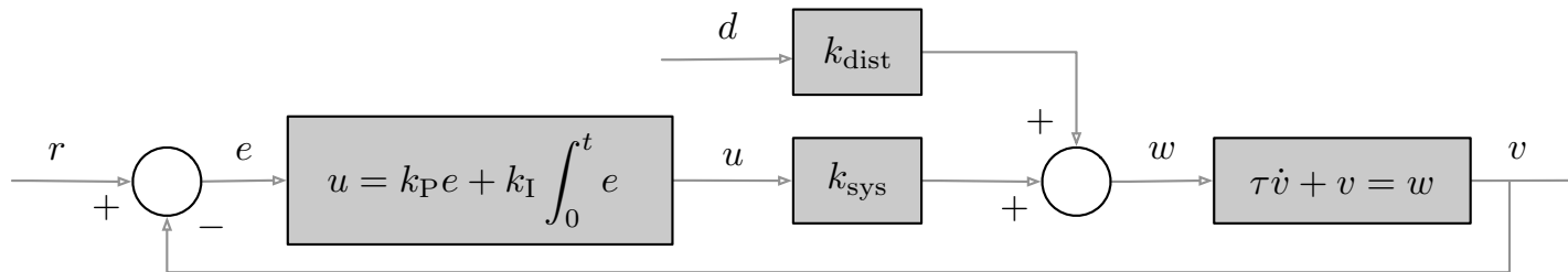
Figure 7.9: Closed-loop PI control of the dynamic car velocity model.
