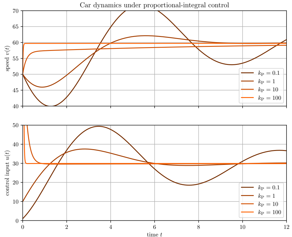
Figure 7.10: Solutions of the cruise-control dynamics with proportional and integral control (7.7): v(t) in the first plot, u(t) in the second plot. The initial velocity is v(0) = 50 and the reference velocity is 60. (The response is from non-zero initial conditions and in response to a step input in r and d .) Multiple values of the proportional control gain k_P and fixed integral gain k_I = 1 .
