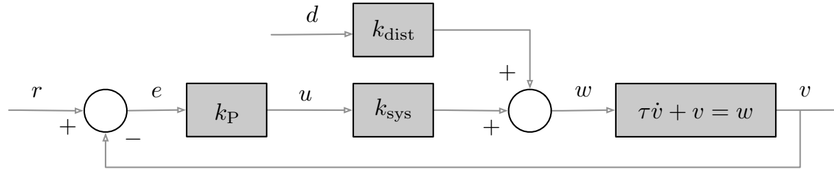
Figure 7.5: Closed-loop P control of the dynamic car velocity model.
