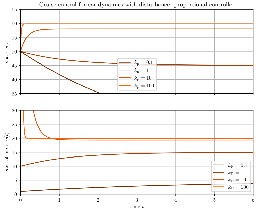
Figure 7.6: Solutions of the cruise control dynamics (7.3): v(t) in the first plot, u(t) in the second plot. The initial velocity is v(0) = 50 and the reference velocity is 60. The closed-loop system is first order; different values of k_p lead to different final values. A larger control gain k_p decreases the time constant and diminishes the steady state error (but no value of k_p achieves perfect regulation with zero steady state error), at the cost of large control signals (see the second plot). Bottom line: none of these solution is satisfactory (even without disturbance d = 0 )
