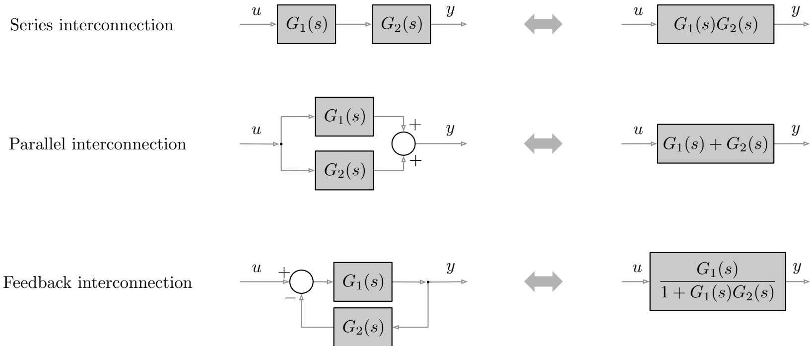
Figure 7.14: The three basic block diagram interconnections in the Laplace domain: series, parallel, and feedback. Each interconnection has an equivalent representation as a single block with equivalent transfer function. These equivalences (and others, e.g., see Exercise E7.8) allow straightforward manipulation of complex block diagrams of transfer functions.
