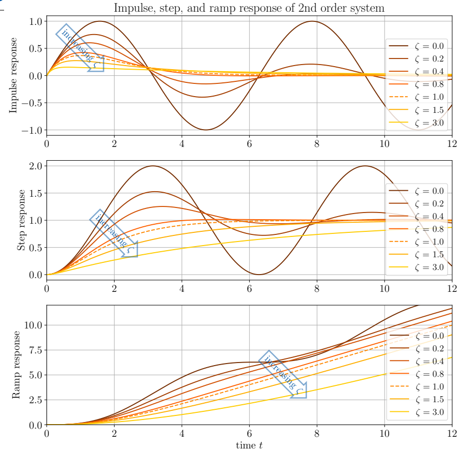
Figure 5.10: Impulse, step, and ramp responses of the 2nd order dynamics (5.19).
