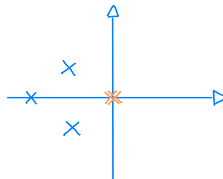
(c) Marginally unstable system : A repeated pole exists on the imaginary axis and every other pole lies in the left half plane. Although all poles are in the left half plane or on the axis, the repeated pole causes unbounded responses.
