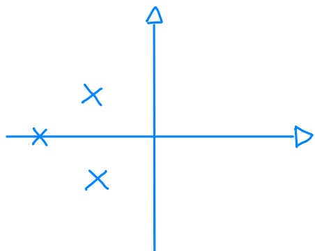
(a) Stable system : All poles lie in the left half of the complex plane. This ensures each system mode decays exponentially over time, resulting in bounded output for any bounded input.
