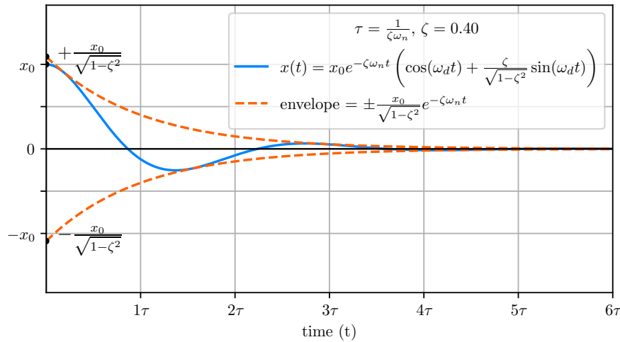
Figure 5.11: Free response of an underdamped second order system from initial position x_0 > 0 and zero initial velocity.
