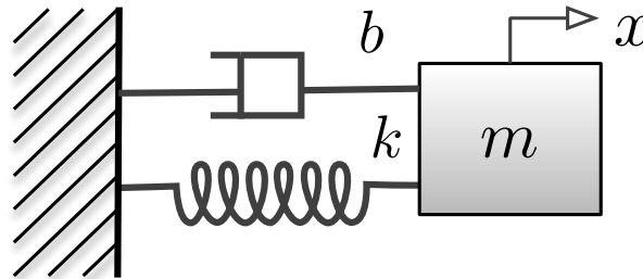
Figure 2.4: A mass-spring-damper system, described by equation (2.12).
