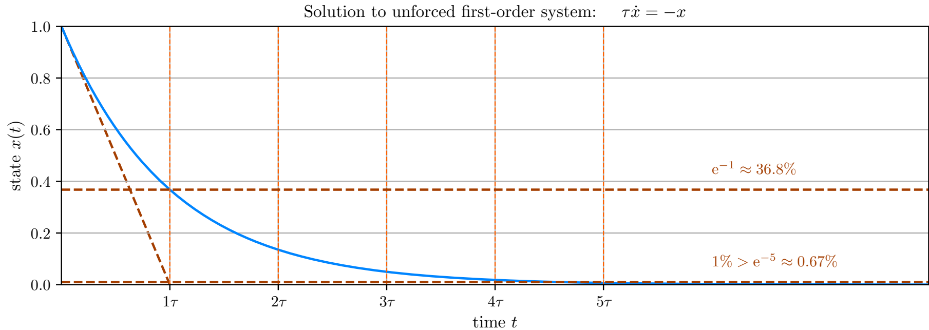
Figure 2.3: Illustrating the time constant of an unforced first-order system \tau \dot{x} = -x , x(0) = 1 .
