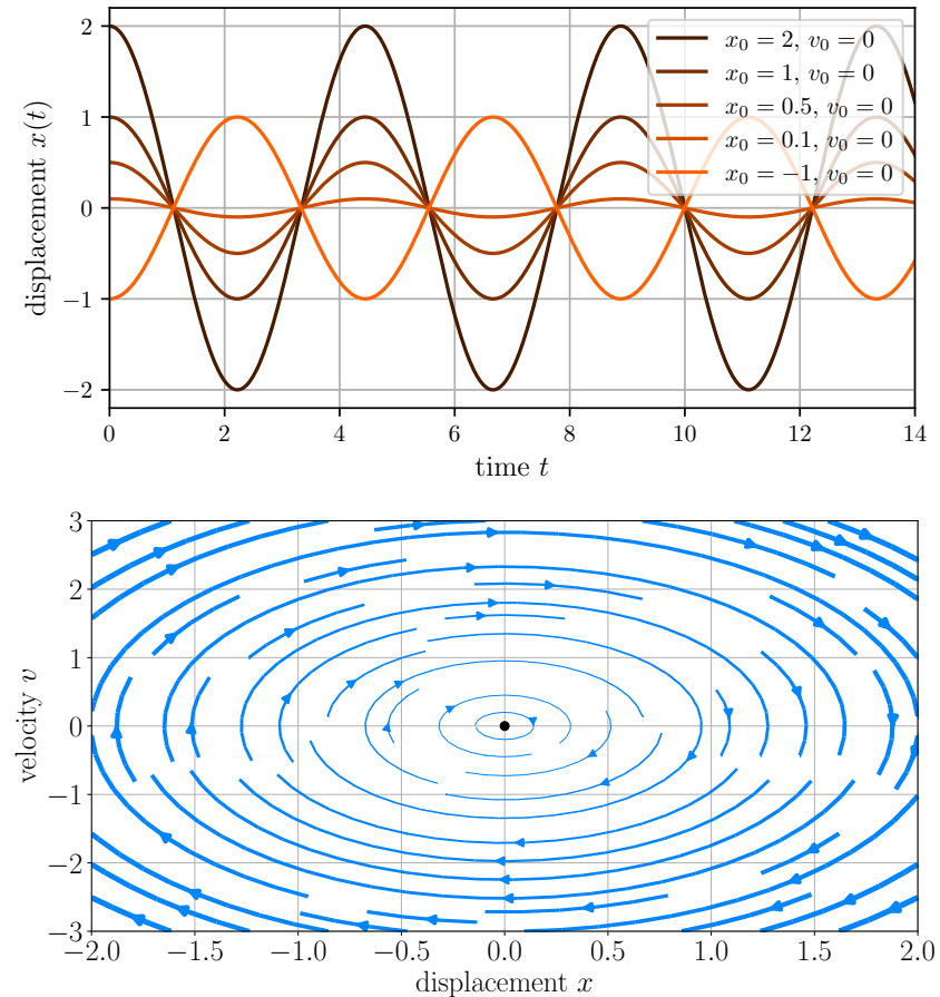
Figure 2.7: Solutions (from zero initial velocity) and phase portrait for the undamped harmonic oscillator (2.15), with m = 1 and k = 2.0 .
