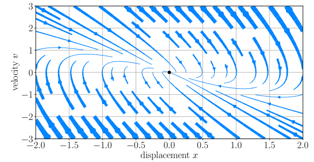
(c) Overdamped system: large b > 0
