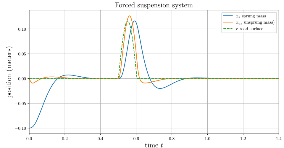
Figure 2.10: Solutions of the suspension system (2.20): unforced solution (road height = 0 for all time) and forced solution due to a speed bump at time 0.5.
