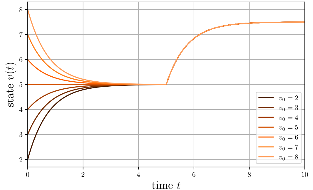
Solutions to the car velocity system
