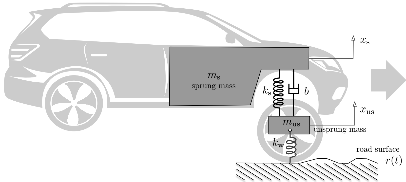
Figure 2.9: The suspension in an automobile.
