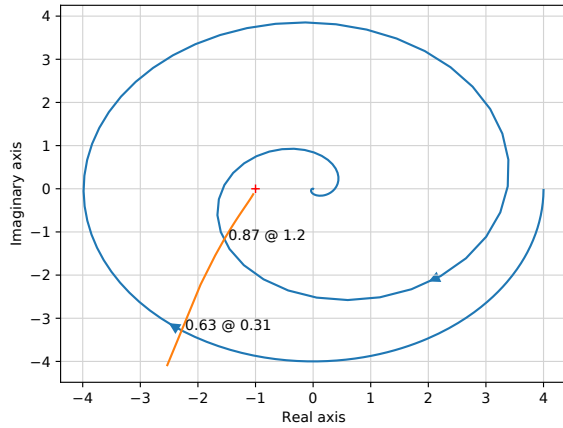
Fig. 2: Polar plot of the frequency response of a describing function.
